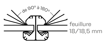
poteau universel 70x70 mm
