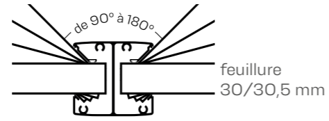
poteau universel 76x70 mm
